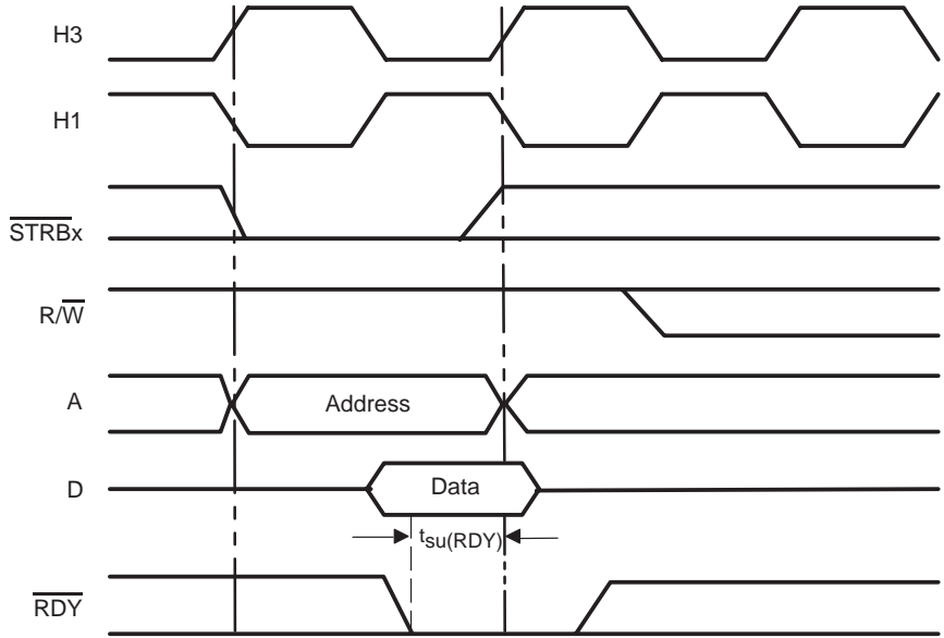
Figure 10–22. \overline{RDY} Timing for Memory Read
