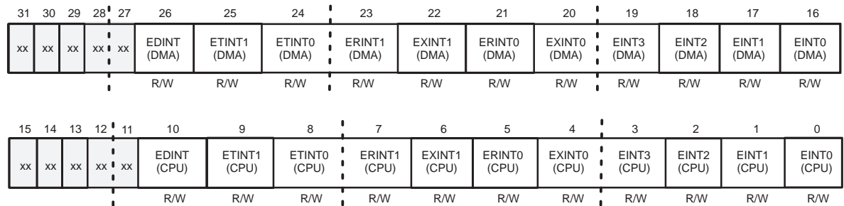
Figure 3–5. CPU/DMA Interrupt-Enable (IE) Register (TMS320C30 and TMS320C31)
