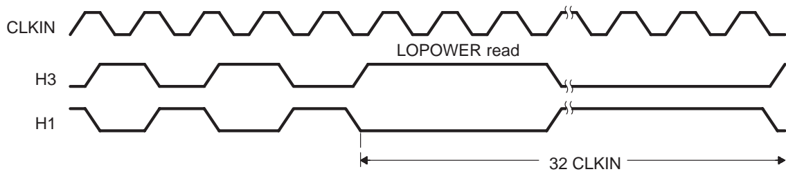
Figure 7–13. LOPOWER Timing
