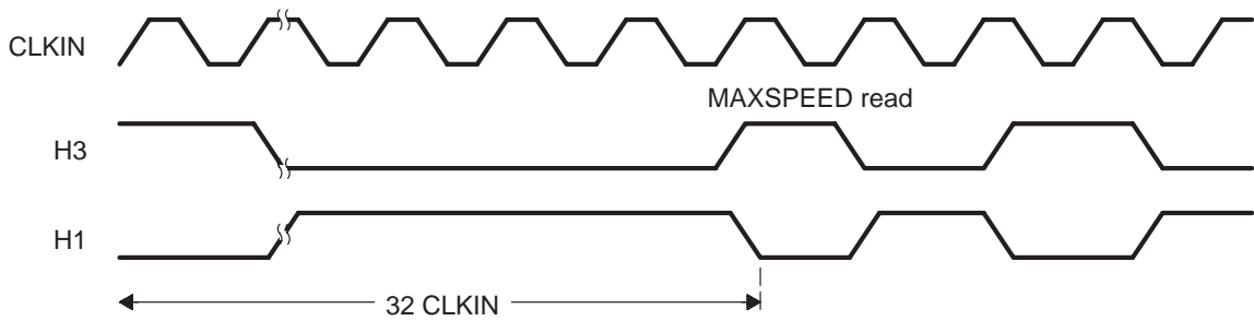
Figure 7–14. MAXSPEED Timing
