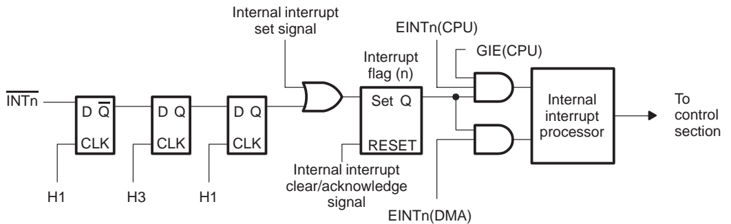
Figure 7–7. Interrupt Logic Functional Diagram
