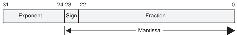
Figure 5–8. Single-Precision Floating-Point Format
