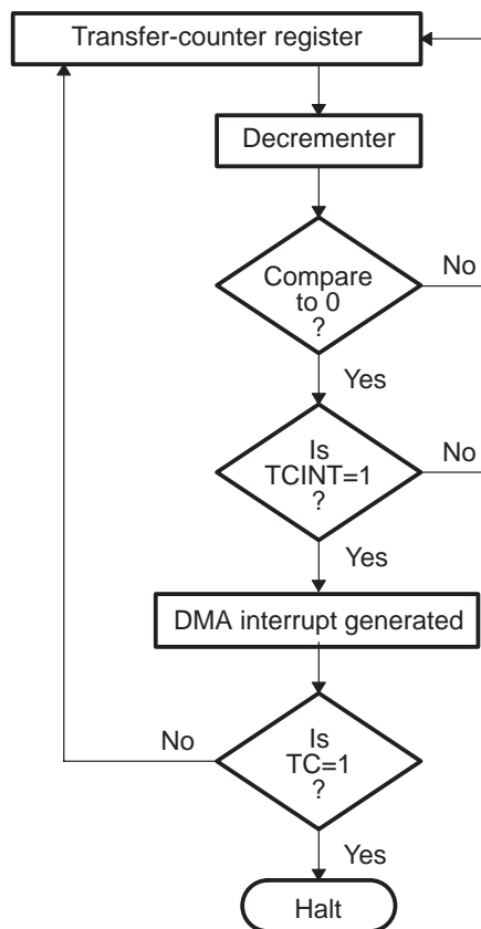
Figure 12–40. Transfer-Counter Operation
