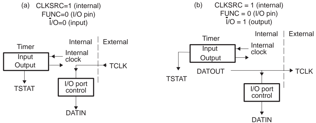
Figure 12–5. Timer Configuration with CLKSRC = 1 and FUNC = 0
