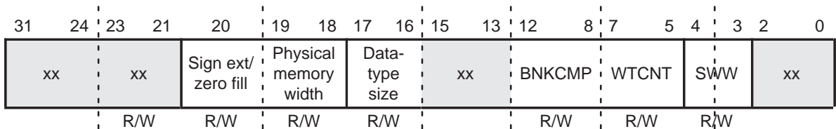
Figure 10–5. \overline{STRB1} Control Register
