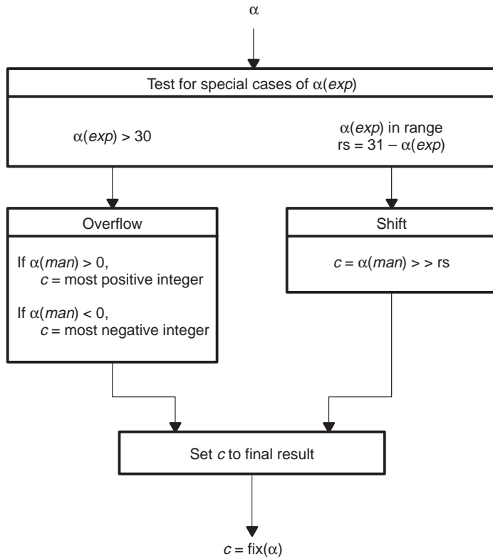
Figure 5–20. Flowchart for Floating-Point to Integer Conversion by FIX Instruction
