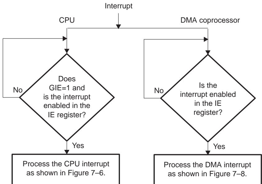
Figure 7–9. Parallel CPU and DMA Interrupt Processing
