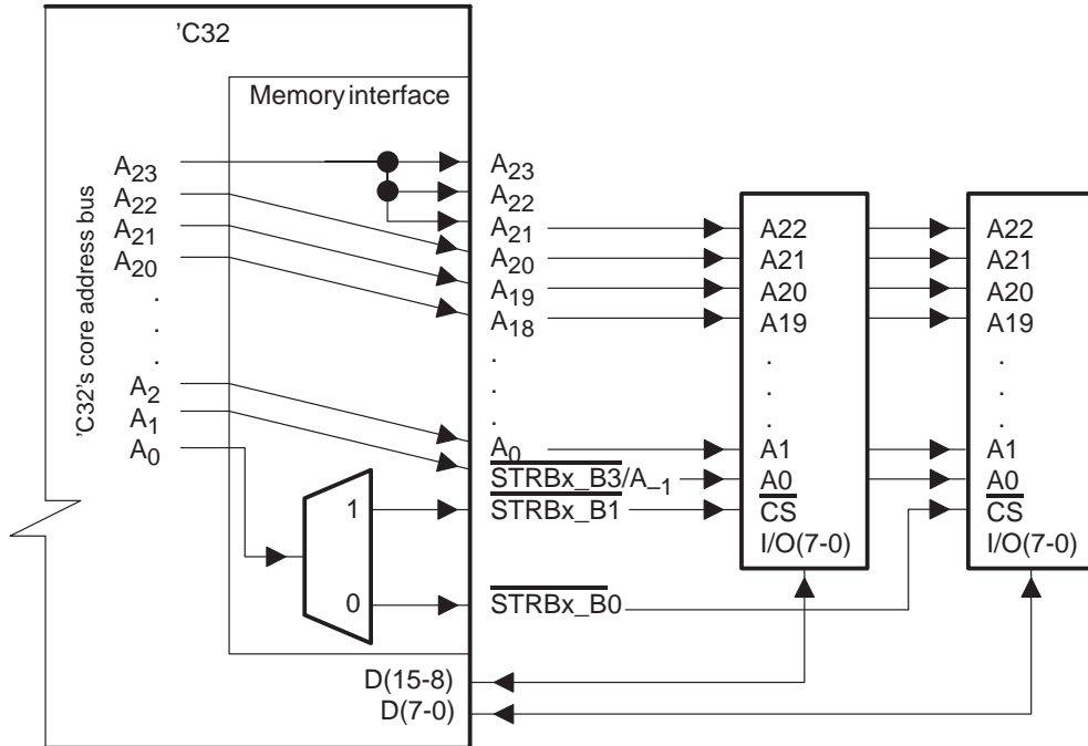
Figure 10–15. Functional Diagram for 8-Bit Data-Type Size and 16-Bit External-Memory Width
