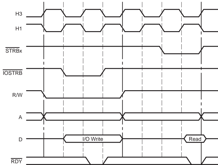
Figure 10–35. \overline{IOSTRB} Write and \overline{STRBx} Read
