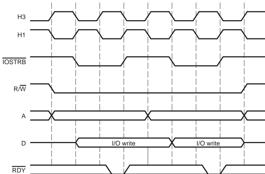
Figure 10–39. \overline{IOSTRB} Write and Write
