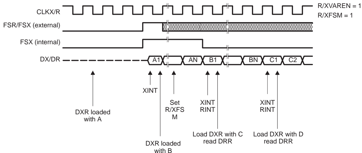
Figure 12–32. Variable Continuous Mode Without Frame Sync
