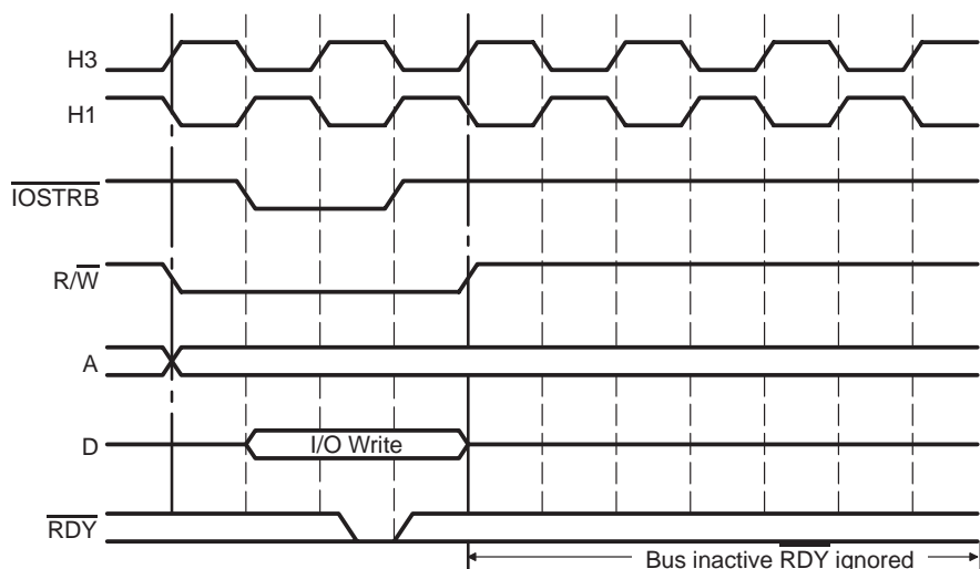
Figure 10–41. Inactive Bus States Following \overline{\text{IOSTRB}} Bus Cycle
