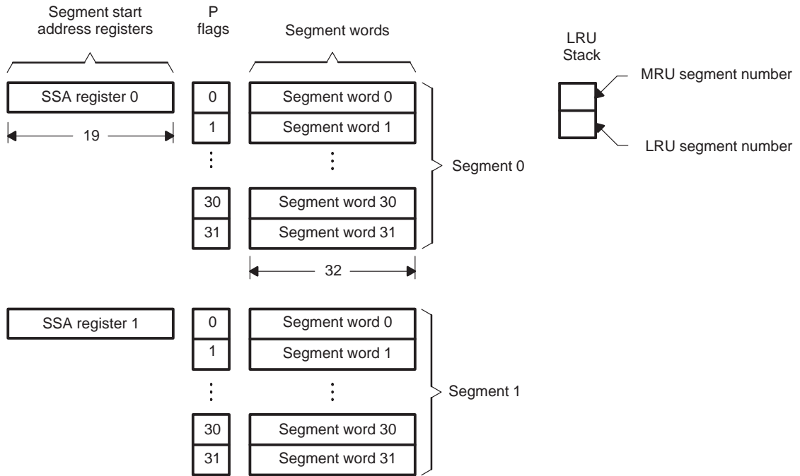
Figure 4–12. Instruction-Cache Architecture
