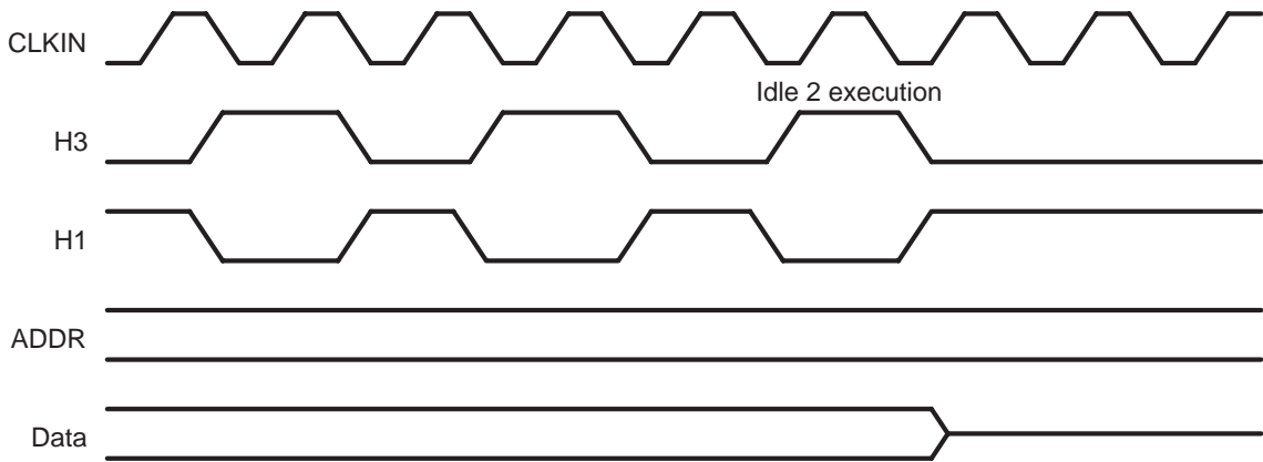
Figure 7–11. IDLE2 Timing
