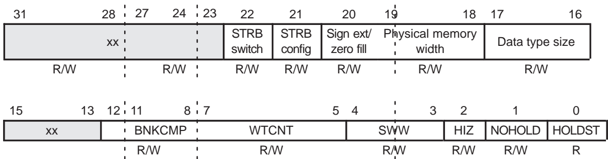
Figure 10–4. \overline{STRB0} Control Register
