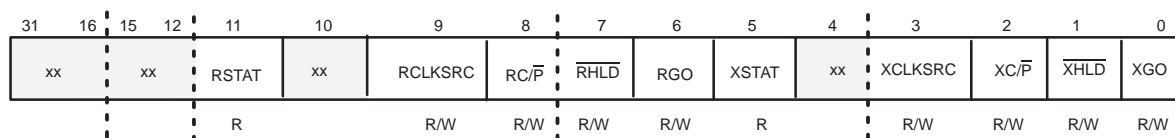
Figure 12–16. Receive/Transmit Timer-Control Register
