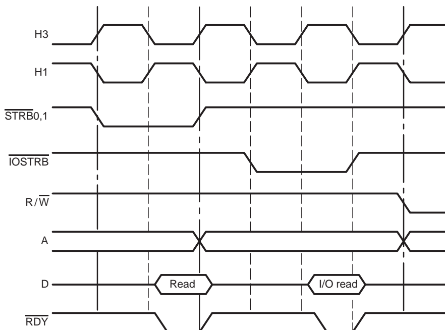
Figure 10–31. \overline{\text{STRB}}_{x,1} Read and \overline{\text{IOSTRB}} Read
