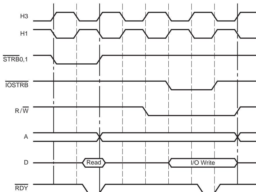
Figure 10–30. \overline{\text{STRB}}_{x,1} Read and \overline{\text{IOSTRB}} Write
