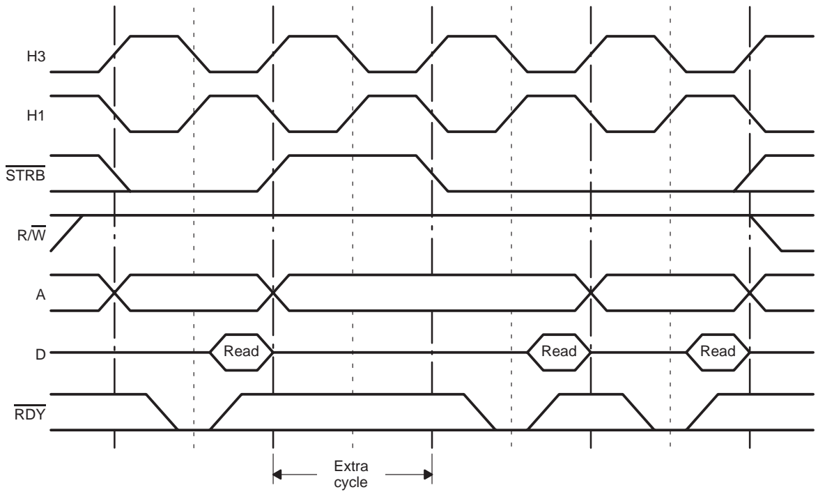
Figure 9–5. Bank-Switching Example
