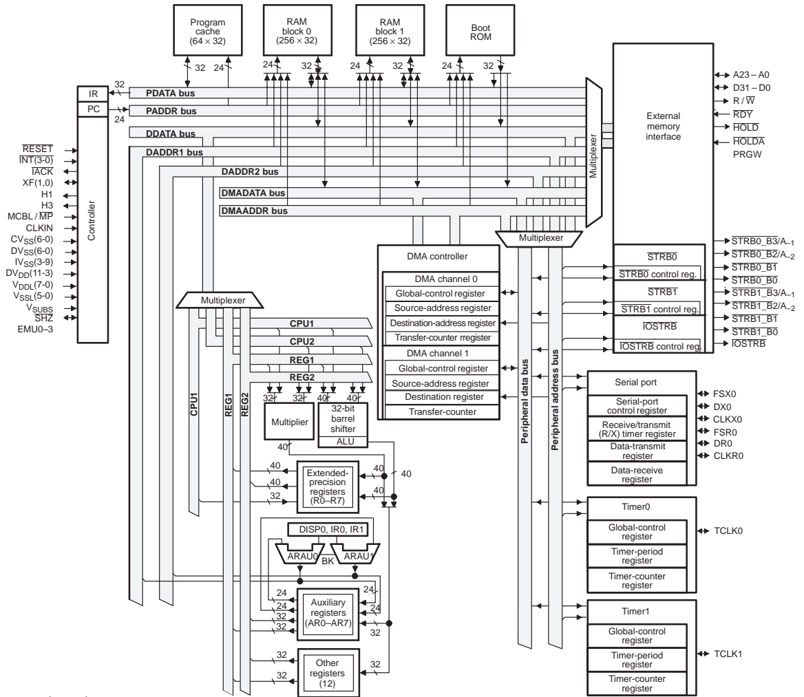
Figure 2–3. TMS320C32 Block Diagram
