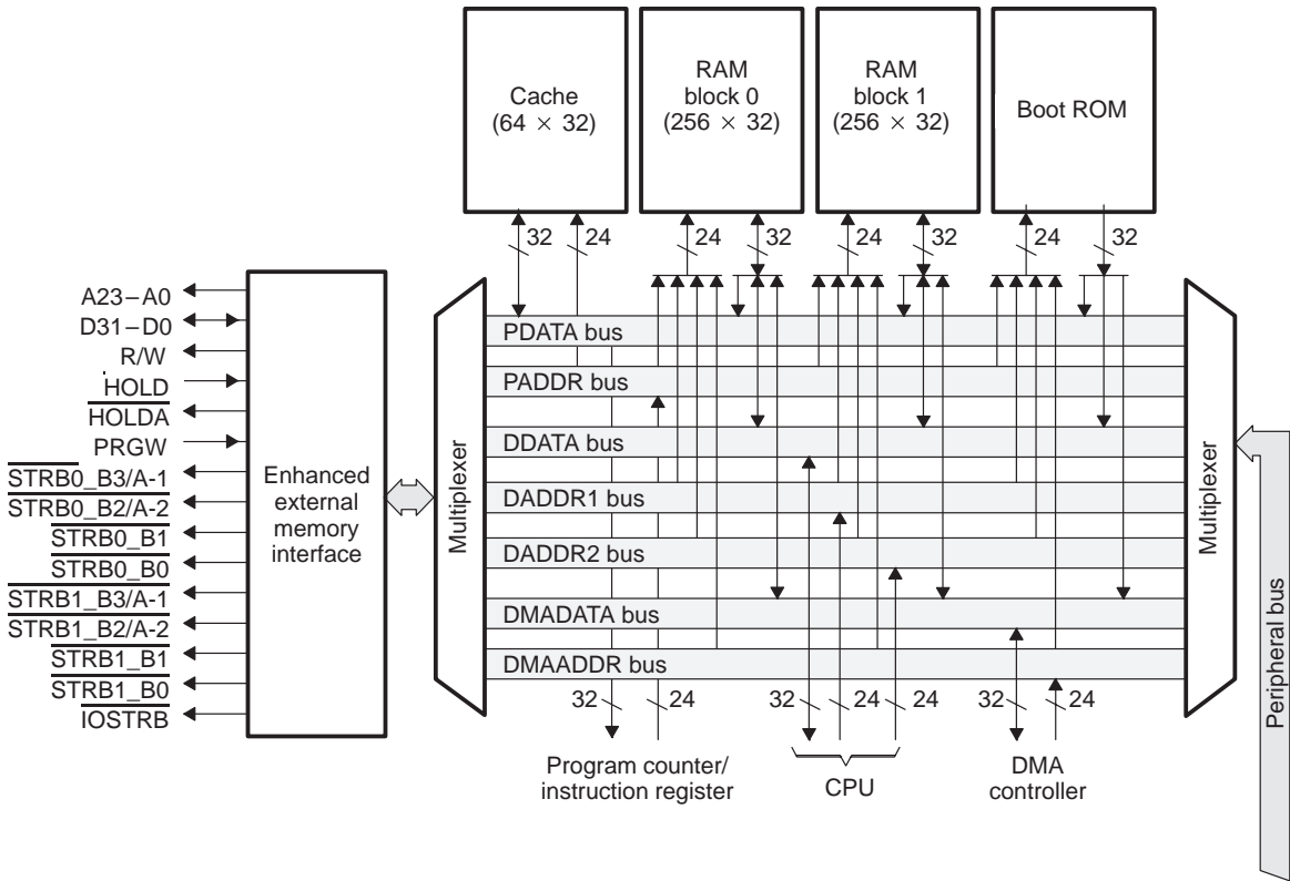
Figure 2–7. Memory Organization of the TMS320C32
