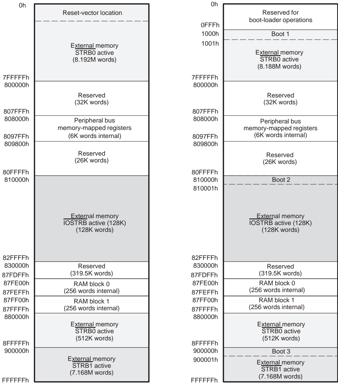
Figure 4–3. TMS320C32 Memory Maps
