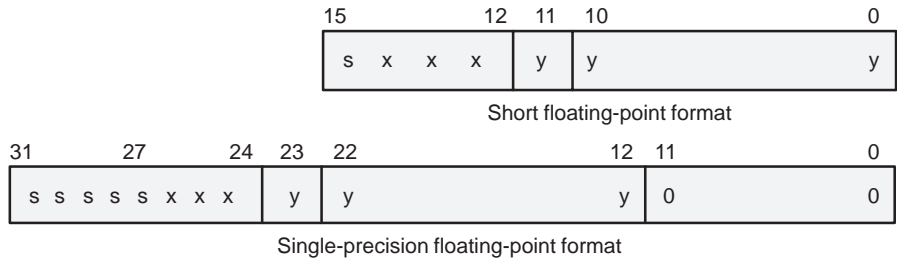
Figure 5–10. Converting from Short Floating-Point Format to Single-Precision Floating-Point Format
