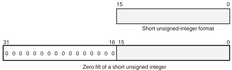
Figure 5–3. Short Unsigned-Integer Format and Zero Fill
