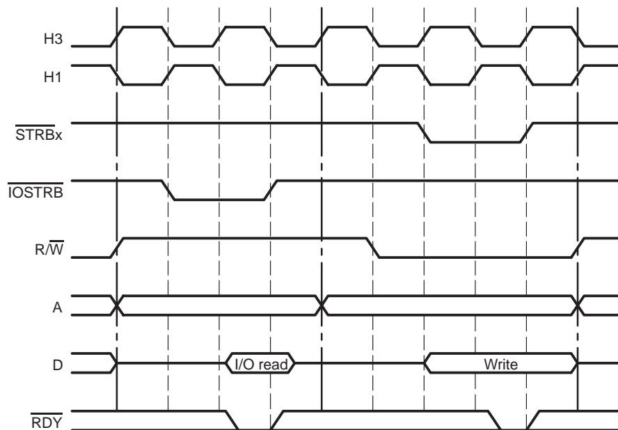
Figure 10–36. \overline{IOSTRB} Read and \overline{STRBx} Write
