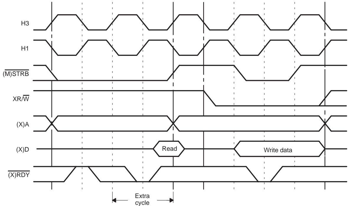
Figure 9–8. Use of Wait States for Read for \overline{(M)STRB} = 0
