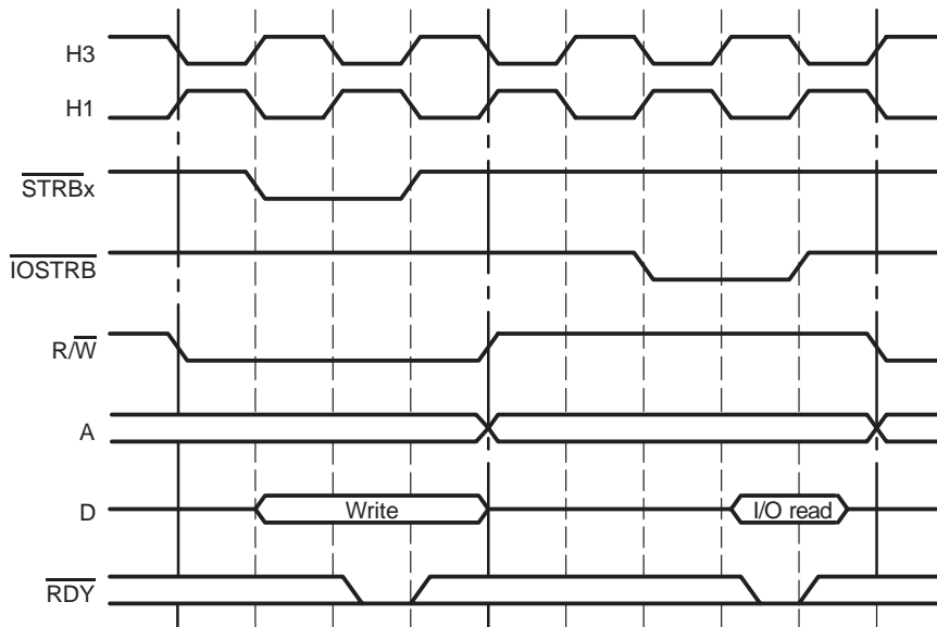
Figure 10–33. \overline{\text{STRBx}} Write and \overline{\text{IOSTRB}} Read
