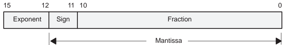
Figure 5–6. Short Floating-Point Format
