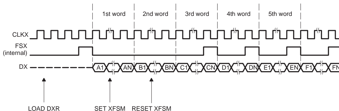
Figure 12–29. Exiting Fixed Continuous Mode Without Frame Sync, FSX Internal
