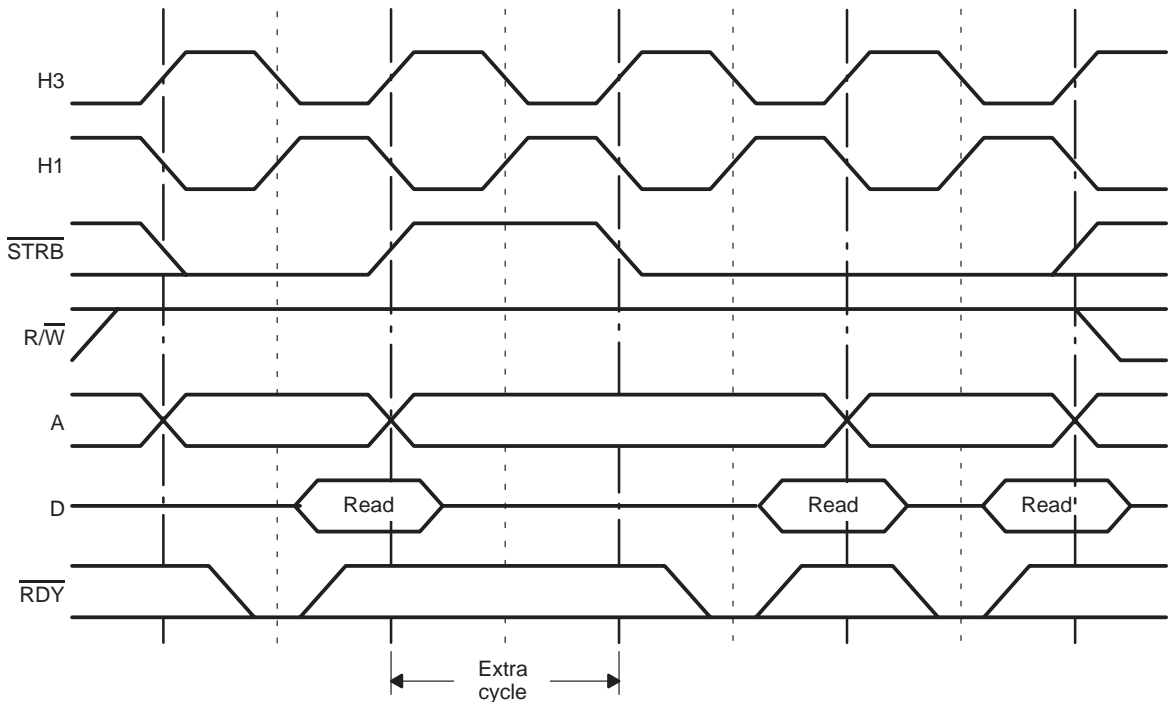
Figure 10–9. Bank-Switching Example
