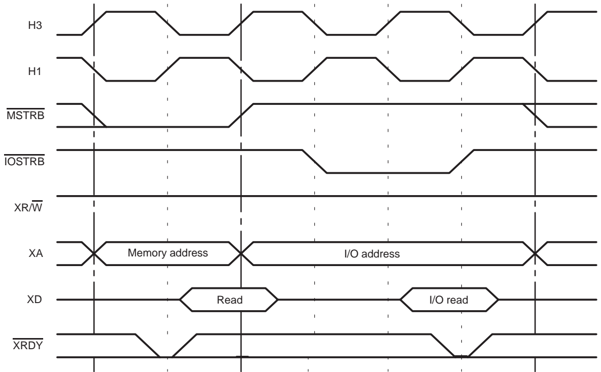
Figure 9–14. Memory Read and I/O Read for Expansion Bus
