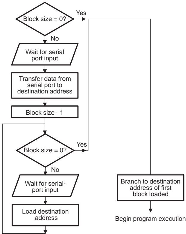
Figure 11–3. Boot-Loader Serial-Port Load-Mode Flowchart
