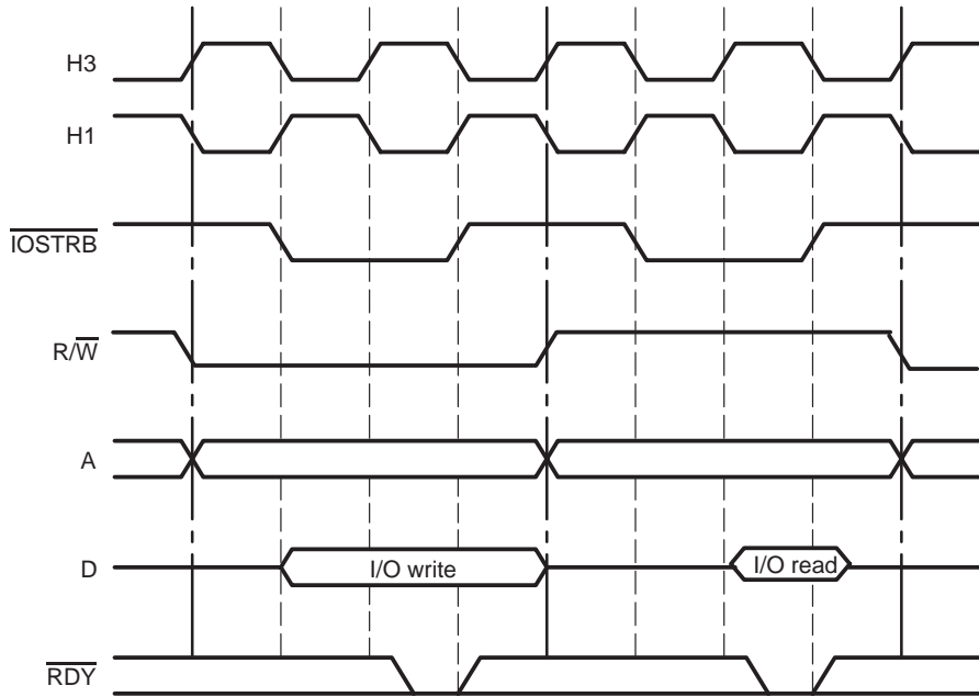
Figure 10–38. \overline{IOSTRB} Write and Read
